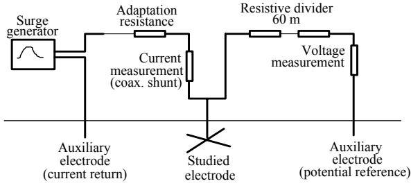
Figure 1: Measuring set-up (adapted from [21]).
