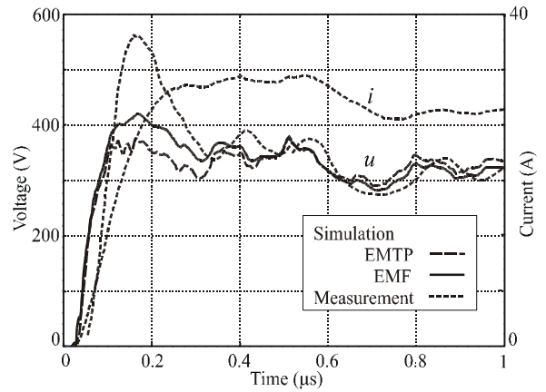
Figure 5: Measurement and simulation of transient voltages to remote ground of double-loop power transmission line tower grounding.
