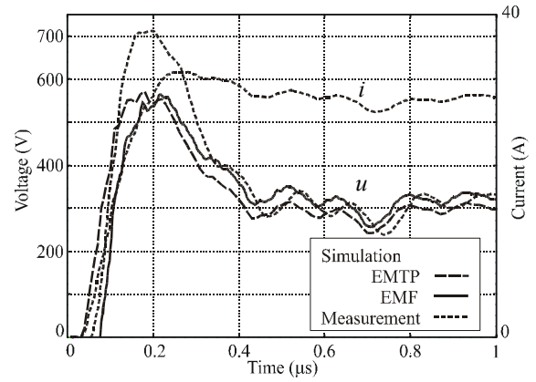
Figure 4: Measurement and simulation of transient voltages to remote ground at the beginning point of 8m long horizontal wire.
