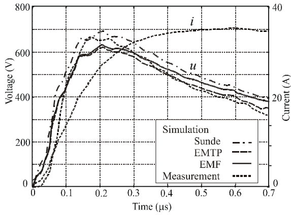
Figure 3: Measurement and simulation of transient voltages to remote ground at the beginning point of 15m long horizontal wire.
