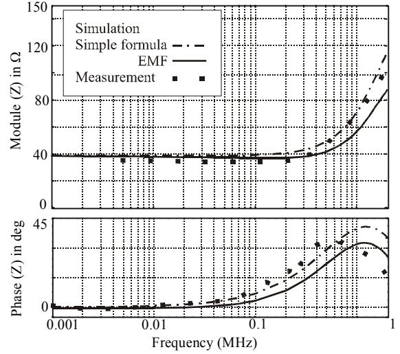
Figure 2: Measurement and simulation of frequency dependent impedance of 16 meters vertical rod electrode.
