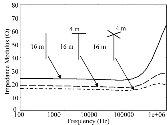
Figure 10. Improved HF impedance of ground rods in soil with \rho = 300 \Omega \cdot m .
