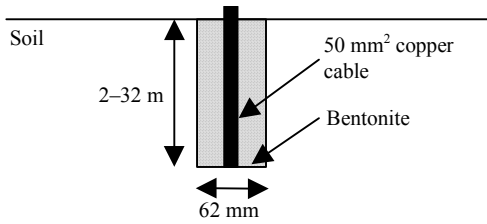
Figure 2. Installation of the measured earth electrode in the ground [1].
