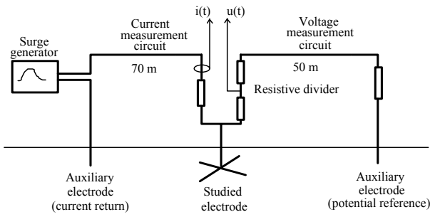
Figure 1. Measuring set-up [1].
