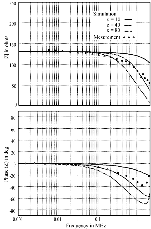
Figure 3. Measurement and simulation of frequency dependent impedance of 4-m rod in soil with \rho = 450 \Omega\cdot\text{m} .
