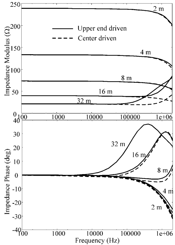
Figure 7. Impedance of ground rods in soil with \rho = 500 \Omega\text{-m} .
