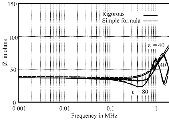
Figure 5. Comparison between rigorous method and simple formulas. Impedance of 16-m rod in soil with \rho = 450 \Omega\text{-m} .
