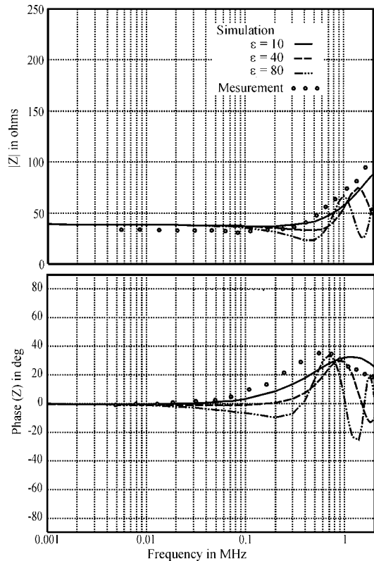
Figure 4. Measurement and simulation of frequency dependent impedance of 16-m rod in soil with \rho = 450 \Omega\cdot\text{m} .
