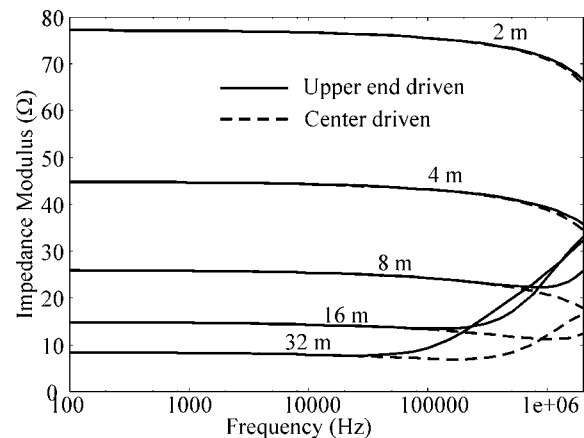
Figure 11. Impedance of two 16-m ground rods at 4-m distance in soil with \rho = 300 \Omega \cdot m .
