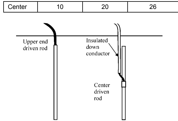
Figure 9. Upper end and center driven rods.
