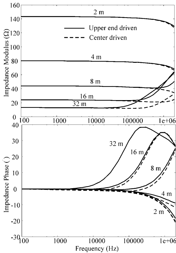
Figure 6. Impedance of ground rods in soil with \rho = 300 \Omega\text{-m} .
