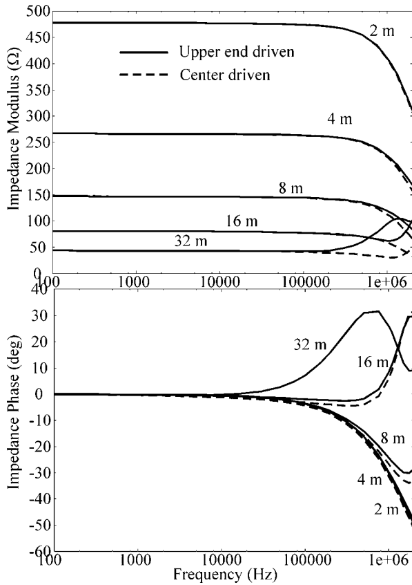
Figure 8. Impedance of ground rods in soil with \rho = 1000 \Omega \cdot m .
